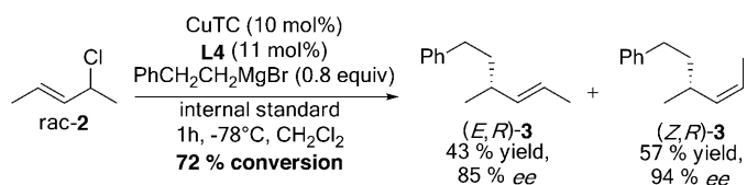
Scheme 4. Control experiment.
